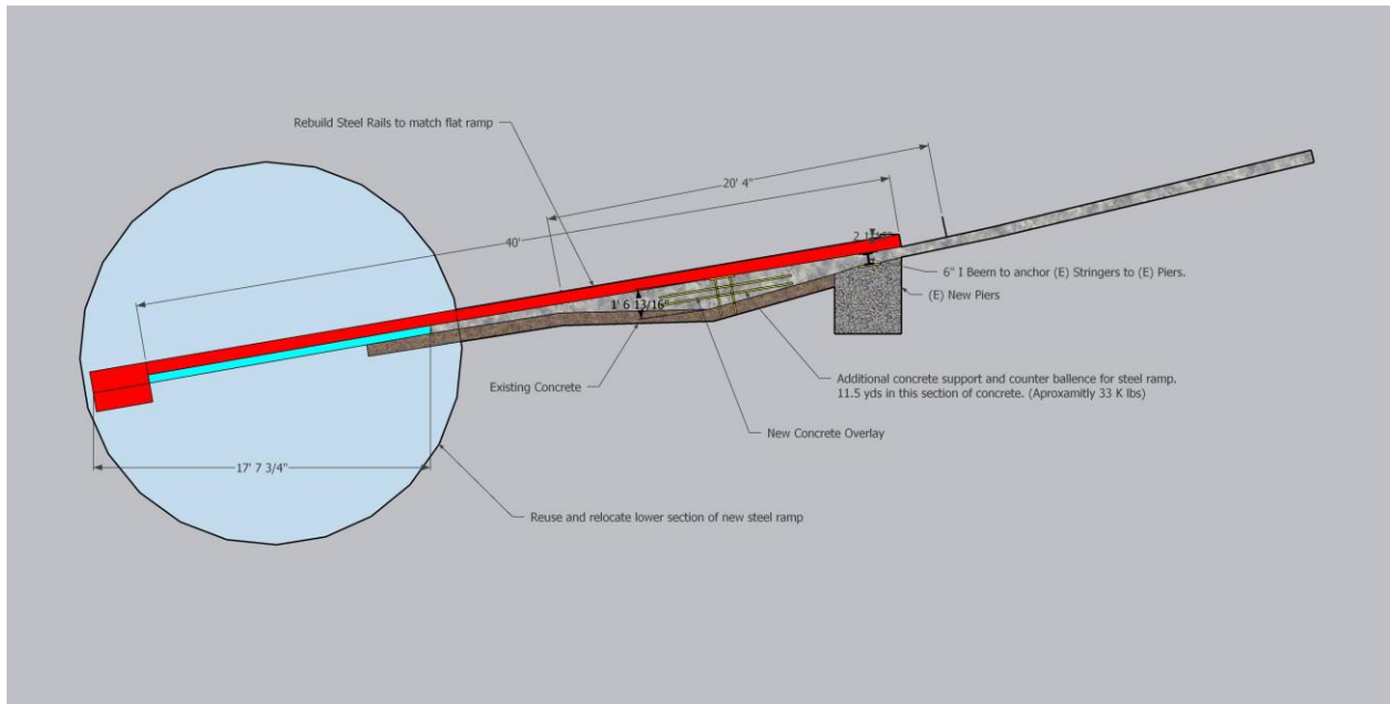
Ramp repair 2024 Concept side-view:
